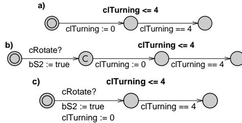
Fig. 3. Delay and sequential composition
